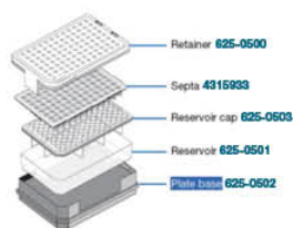
Water/Waste Reservoir Assembly
