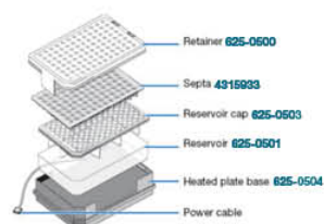
Buffer Reservoir Assembly
